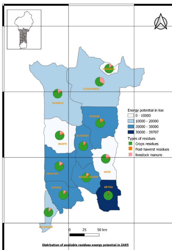
Fig. 6. Distribution of available residue energy potential in ZAE5
