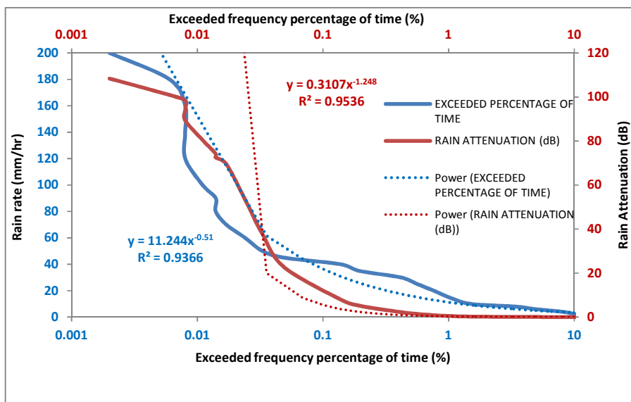
Fig. 3. Relationship between frequency percentage time and rain attenuation for August 2017
