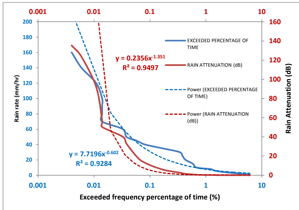
Fig. 4. Relationship between frequency percentage time and rain attenuation for October 2017
