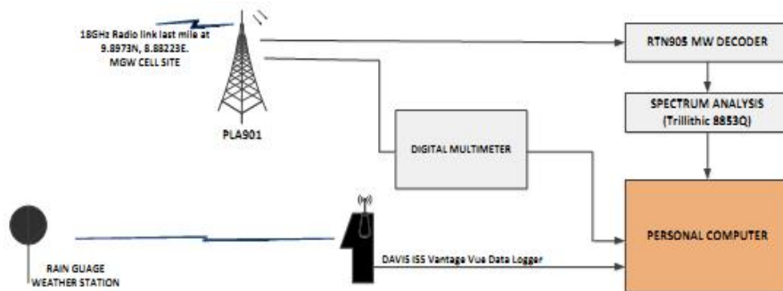
Fig. 1. Experimental setup
