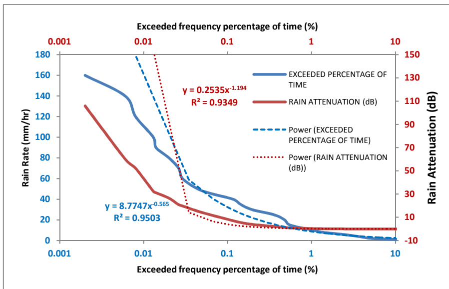
Fig. 2. Relationship between frequency percentage time and rain attenuation for July 2017
