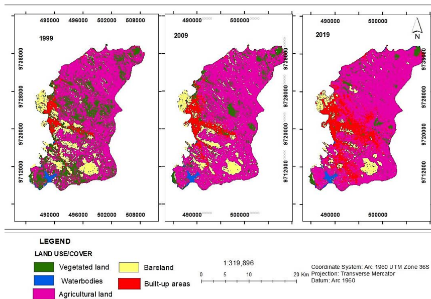
Fig. 1. The 1999, 2009 & 2019 classified LULC maps
