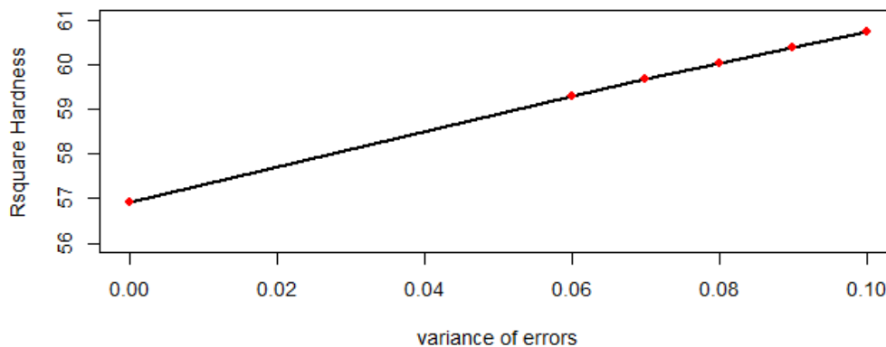
Fig. 2. Graph of R-square against error variances for hardness
