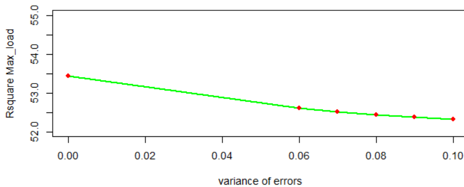
Fig. 1. graph of R-square values against error variances for the maximum load
