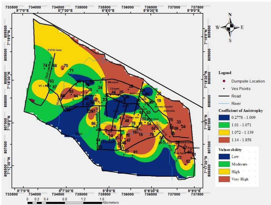
Fig. 9. Coefficient of anisotropy map of FUTA campus
