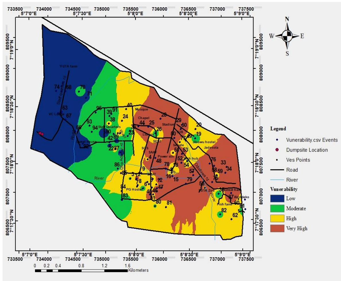
Fig. 10. Aquifer vulnerability model map of FUTA campus
