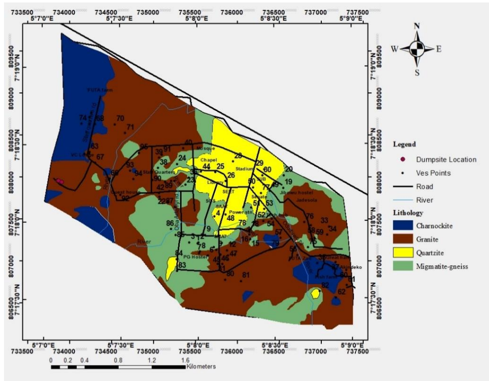
Fig. 3. Geological map of the study area [11]
