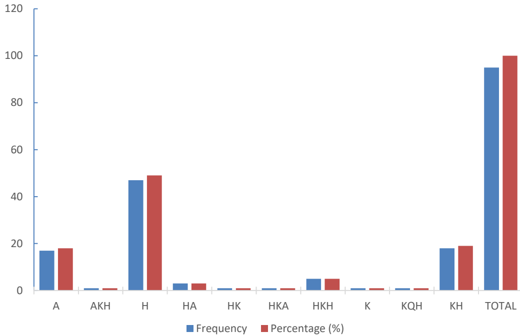
Fig. 5. The frequency of the curve type obtained from the FUTA Campus
