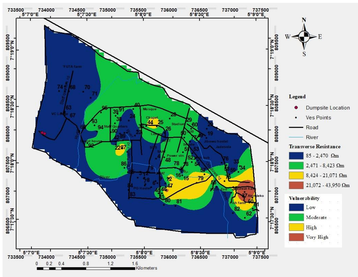
Fig. 7. Transverse resistance map of FUTA campus
