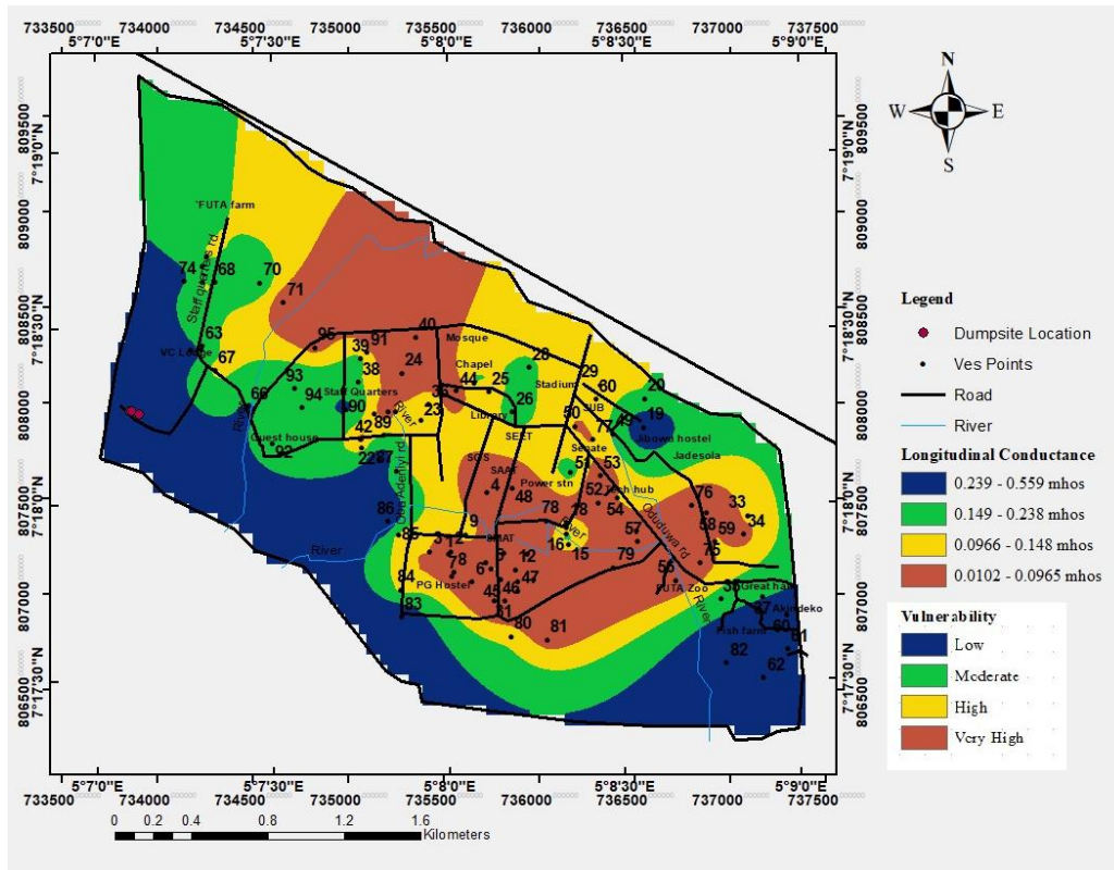
Fig. 8. Longitudinal conductance map of FUTA campus
