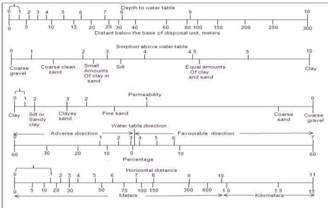
Fig. 4. Le Grand pollution chart [12]
