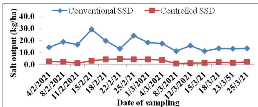
Fig. 5. Temporal variations in salt removal ( \text{kg ha}^{-1} ) as influenced by conventional and controlled SSD at 50 m lateral spacing during R/S 2020-21
