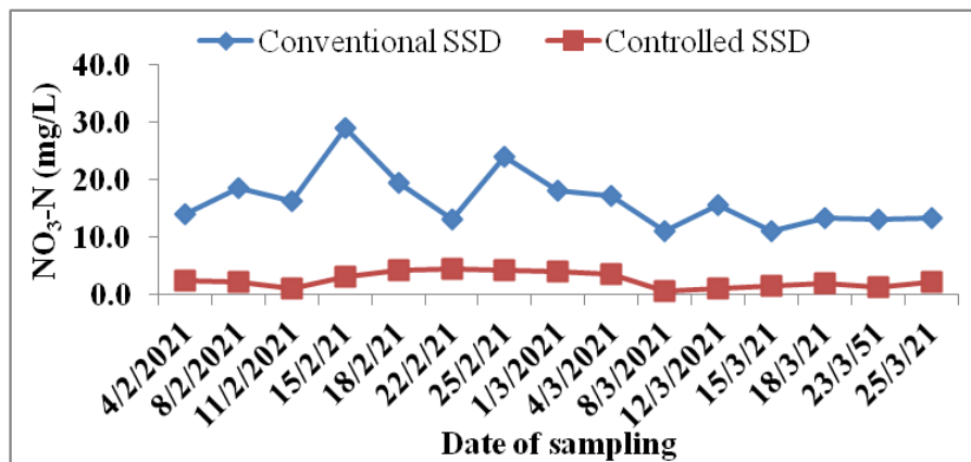
Fig. 6. Temporal variations of NO 3 -N concentrations (mg L -1 ) in drain discharge water as influenced by conventional and controlled SSD at 50 m lateral spacing during R/S 2020-21
