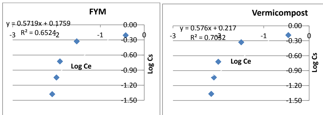
Fig. 5. Freundlich Sorption isotherm of atrazine as influenced by the various organic amendments
