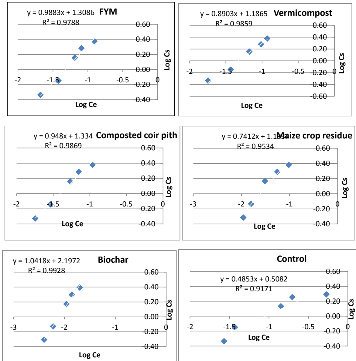
Fig. 4. Freundlich Sorption isotherm of pendimethalin as influenced by the various organic amendments
