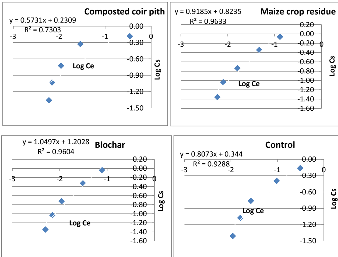
Fig. 6. Freundlich Sorption isotherm of imazethapyr as influenced by the various organic amendments
