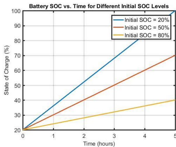
Fig. 9. SOC vs. time for different initial SOC levels
