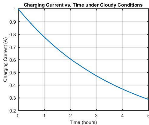
Fig. 8. Charging current vs. time under cloudy conditions
