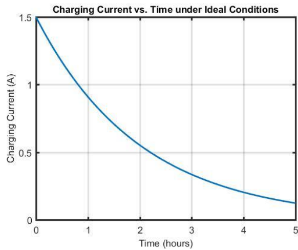
Fig. 5. Charging current vs. time under ideal conditions
