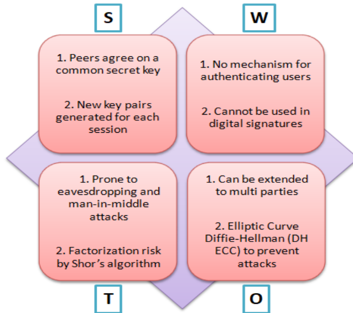
Fig. 10. SWOT analysis of Diffie-Hellman
