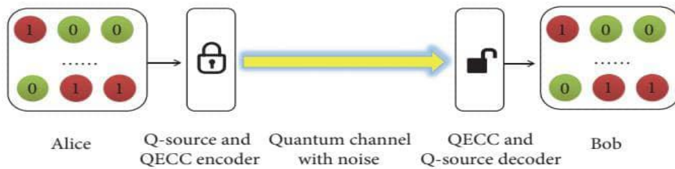
Fig. 4. Quantum direct transmission model
