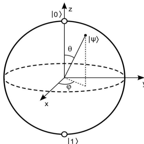
Fig. 1. The Bloch sphere showing the geometrical representation of a qubit
