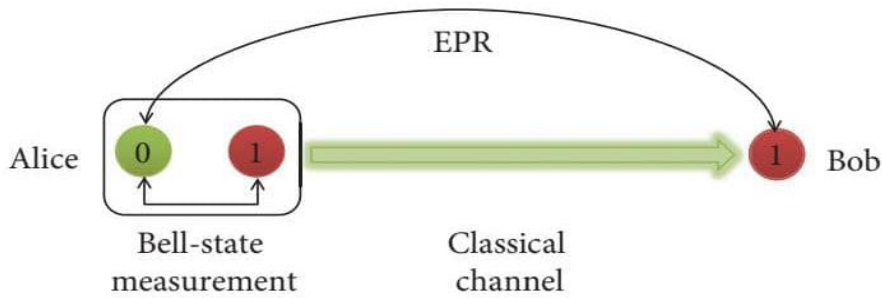
Fig. 3. Illustration of the quantum teleportation model
