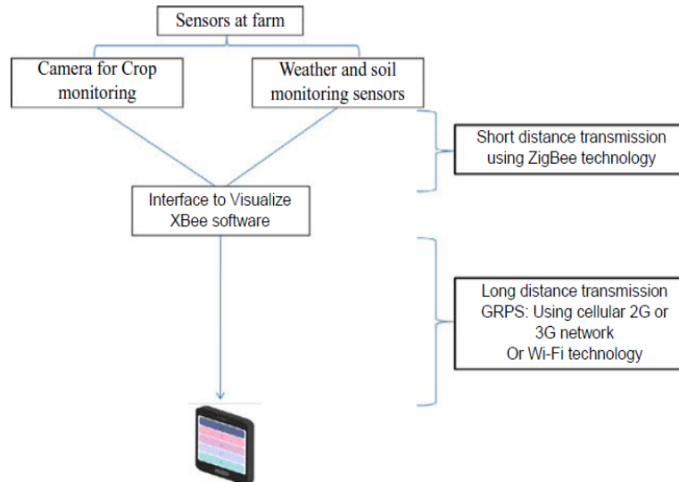
Fig. 3. An application of Wi-Fi modules and circuitry design of sensors for automated irrigation. [7]
