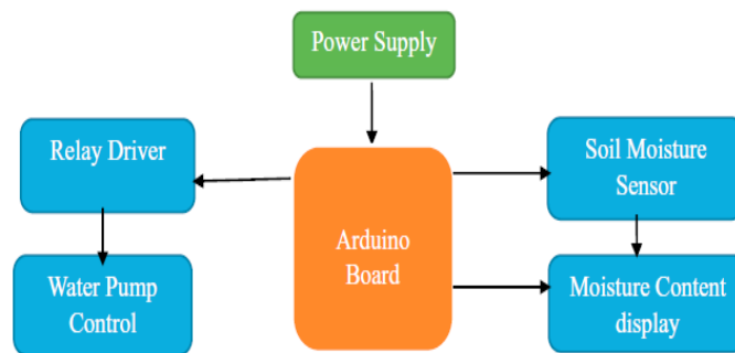
Fig. 4. IoT-based automation process. (Source: Modified and updated from Jha, K., Doshi, A., Patel, P., 2018)
