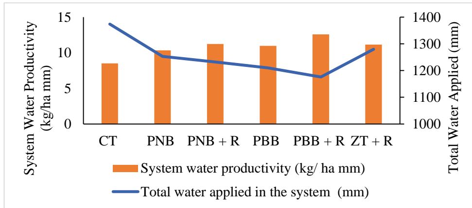
Fig. 6. Impacts of tillage, bed planting and residue management on water productivity of cotton-wheat system
