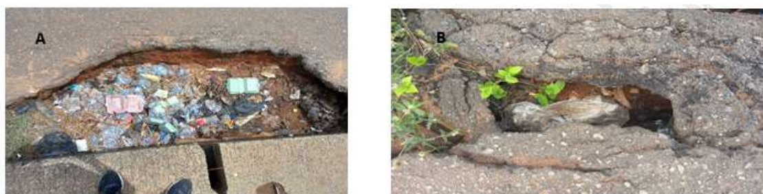
Fig. 2. (a) Sinkhole at Awka site 1 (b) Soil pipe at Awka site 2 Geology and Global Information System of Anambra state
