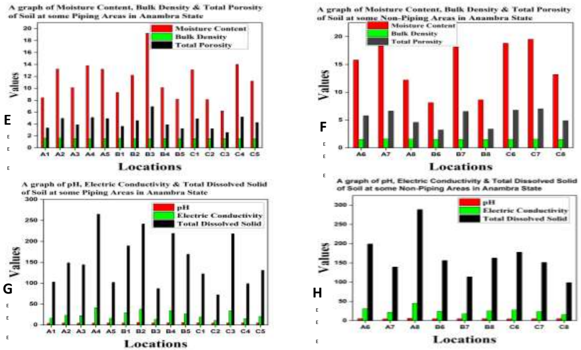
Fig. 4. (a) A graph soil texture at the piping area (b) A graph of soil texture at the non-piping area (c) A graph of OM, OC and K_F at the piping area (d) A graph of OM, OC and K_F at the non-piping area (e) A graph of MC, D_B and P_t at the piping area (f) A graph of MC, D_B and P_t at the non-piping area (g) A graph of pH, EC and TDS at the piping area (h) A graph of pH, EC and TDS at the non-piping area
