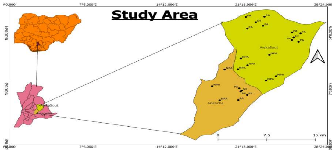
Fig. 1. The study area with an insert of Anambra state and Nigeria (SH = Sinkholes, PA = Piping Area, NPA = Non-piping area)
