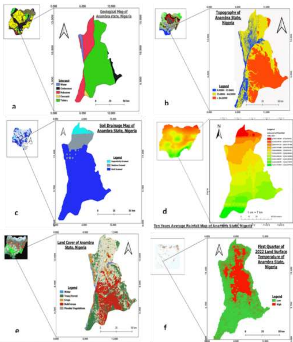
Fig. 3. (a) Geological map of Anambra state (b) Topography map of Anambra state (c) Soil drainage map of Anambra state (d) 10 years average rainfall of Anambra state (e) Land cover map of Anambra state (f) First quarter of 2022 land surface temperature map of Anambra state
