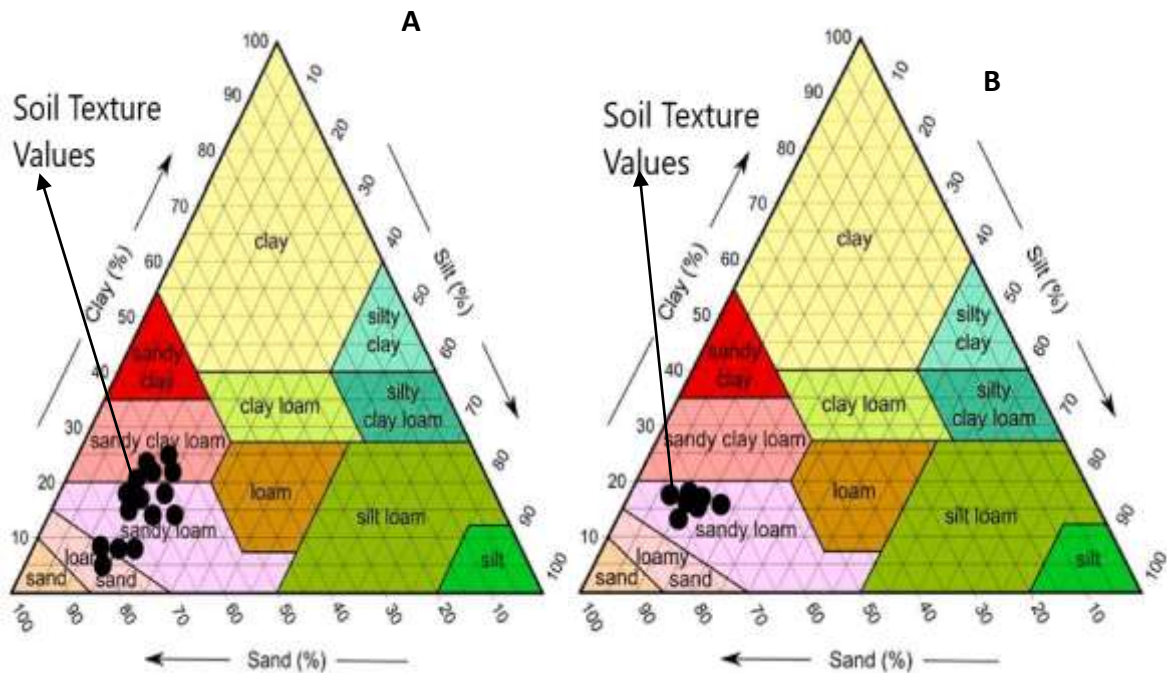
Fig. 5. (a) Ternary graph for soil texture class at the piping area (b) Ternary graph for soil texture class at the non-piping area
