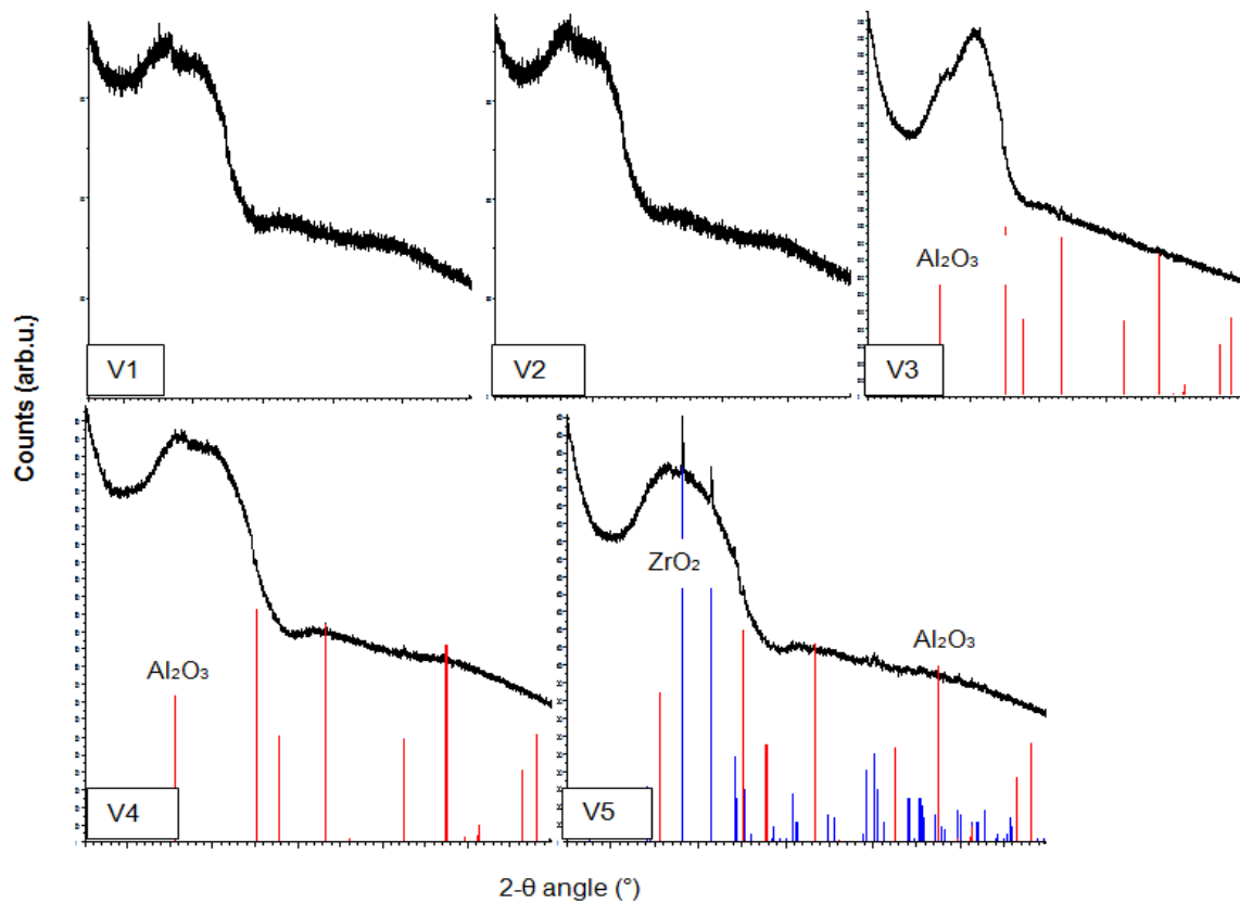
Fig. 3. XRD spectra of alkali-resistant glasses V1, V2, V3, V4 and V5
