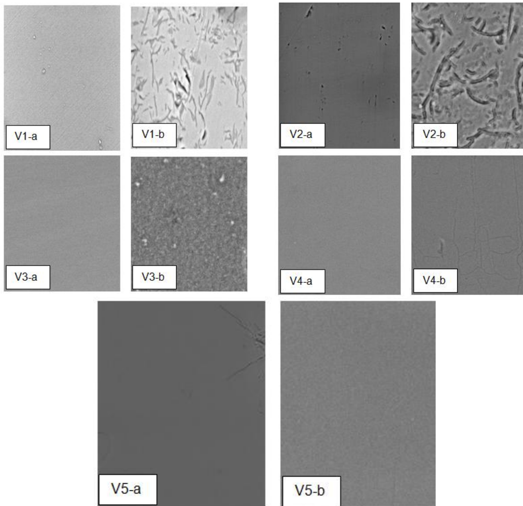
Fig. 5. SEM images ( \times 700 ) of V1, V2, V3, V4 and V5 glasses: a) unaltered glasses b) altered glasses after dipping in a alkaline solution of NaOH at pH=13 and 90°C for 28 days
